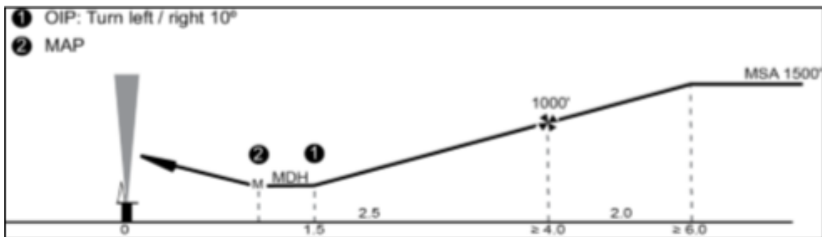
Figure 2 — Vertical profile
